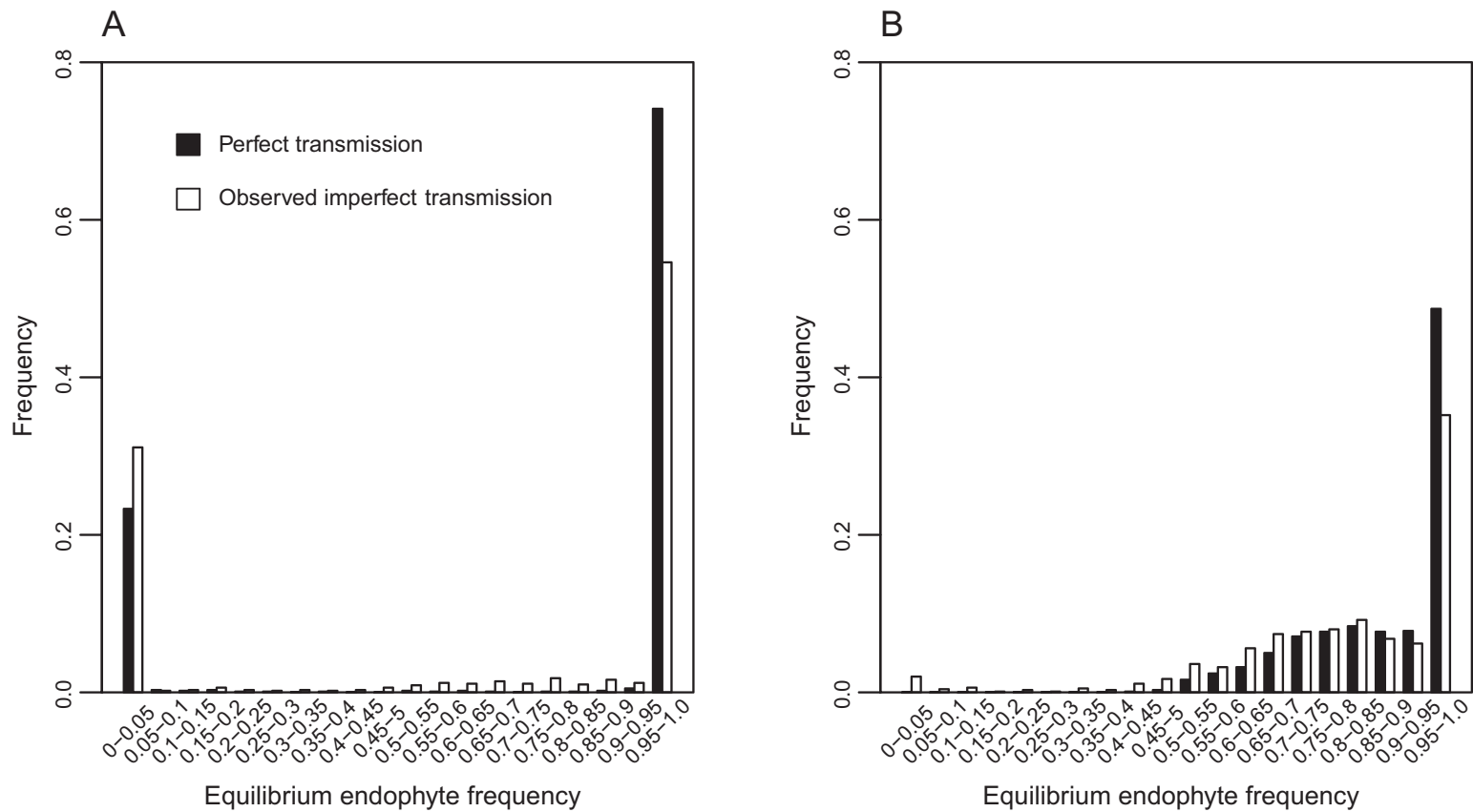
Figure 3: Histograms of equilibrium endophyte frequency in which parameter values were estimated from 1,000 bootstrap replicates (parameter distributions shown in fig. 2). Black bars show results assuming perfect vertical transmission of endophytes, and white bars show results based on observed transmission rates. A , Niche differences removed ( \alpha^- = \alpha^+ = 1 ) with all other parameters drawn from uncertainty ranges. B , Observed niche differences included ( \alpha 's drawn from uncertainty ranges).
